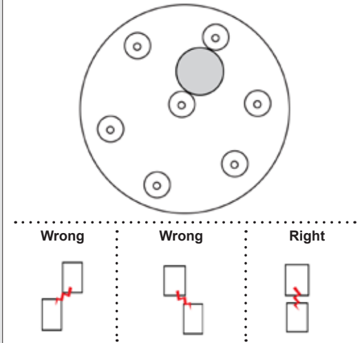
Cap & Rotor indexing by drilling a hole in an old cap and align the contact properly. This may take some tweaking to get the best alignment.
