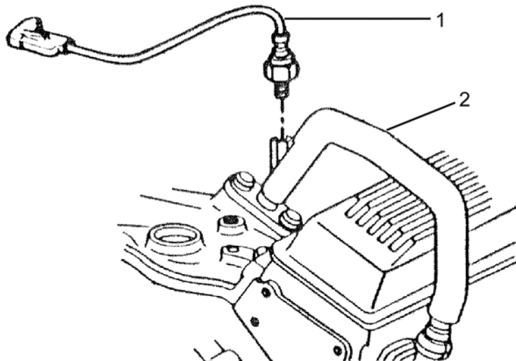
1-EGR Temperature Diagnostic Switch 2-EGR Pipe Shield
